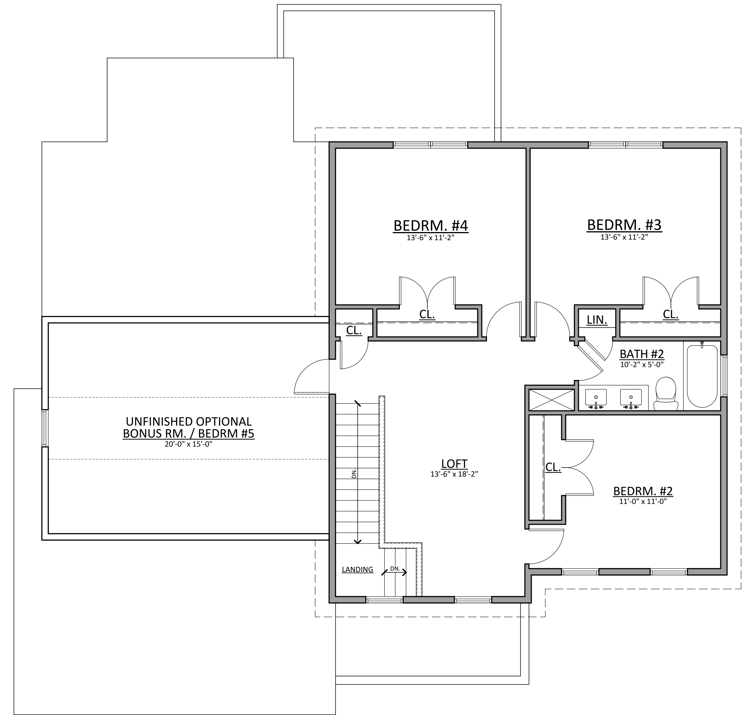
UPPER LEVEL FLOOR PLAN
