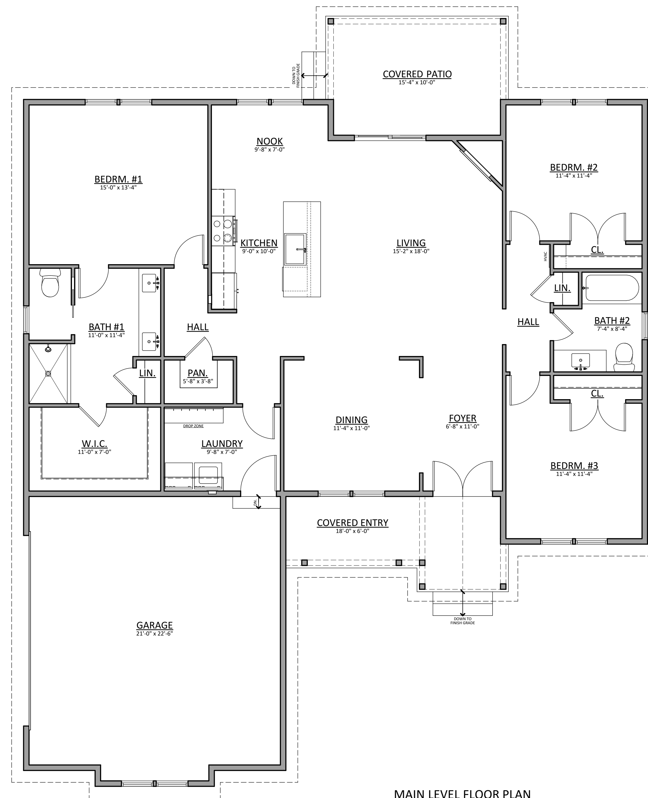
MAIN LEVEL FLOOR PLAN N.T.S.
