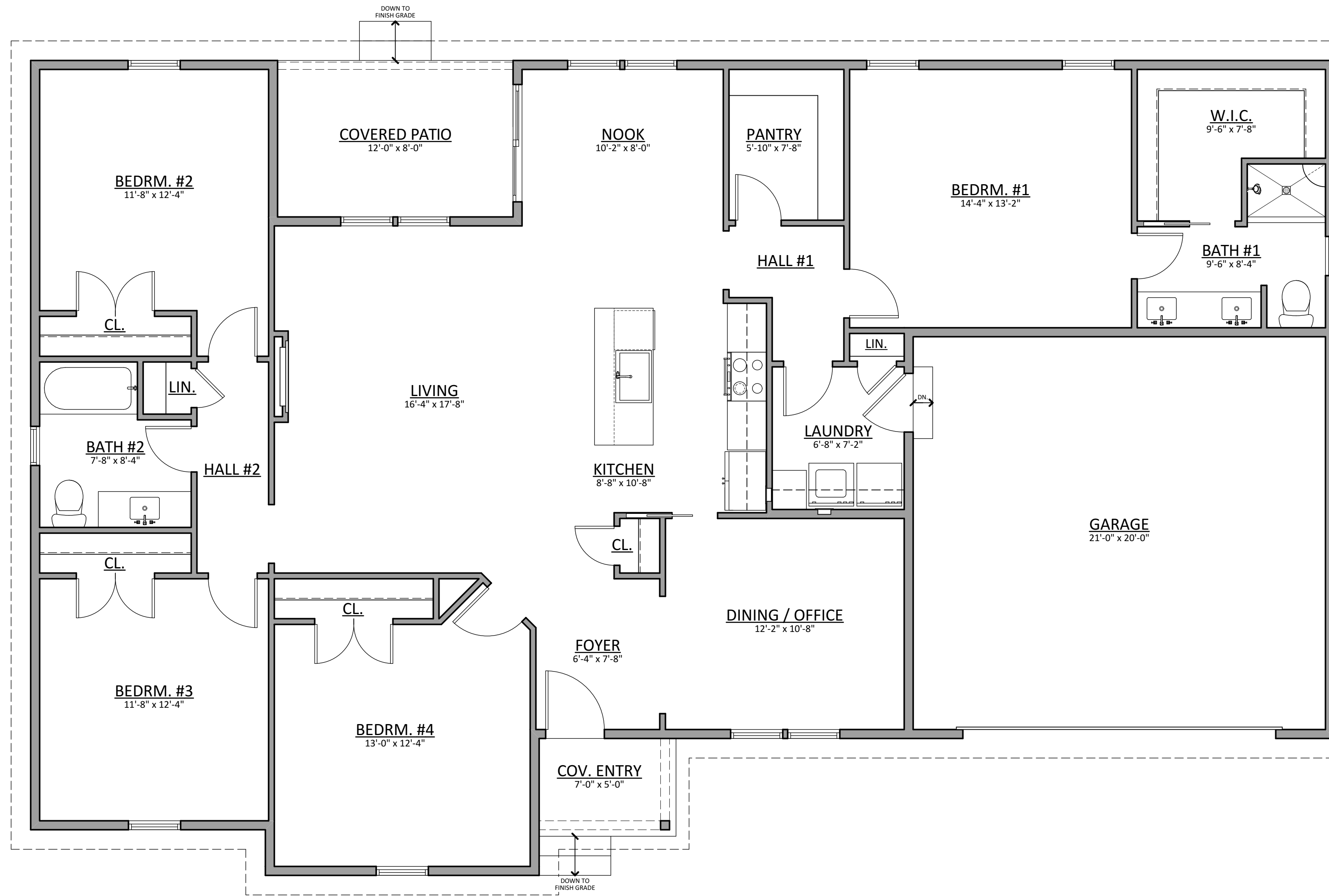
MAIN LEVEL FLOOR PLAN N.T.S
